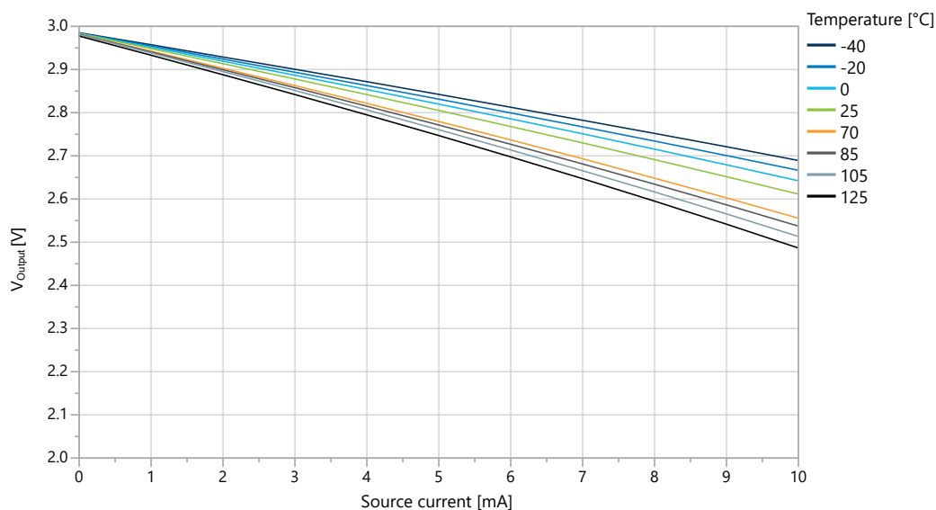
Figure 38-22. I/O Pin Output Voltage vs. Source Current ( V_{\text{DD}} = 3.0\text{V} )
