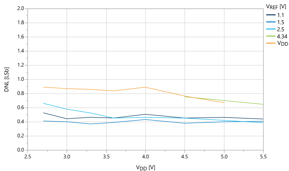
Figure 38-38. DNL Error vs. V_{DD} ( f_{ADC} = 115 kps) at T = 25^{\circ}C , REFSEL = Internal Reference
