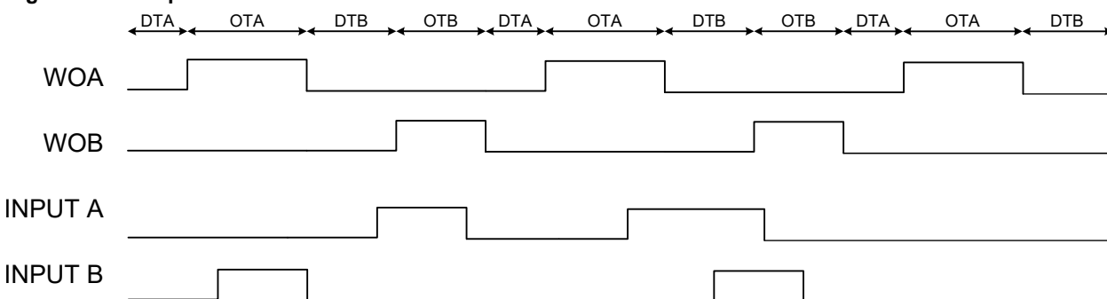
Figure 23-10. Input Mode 0
