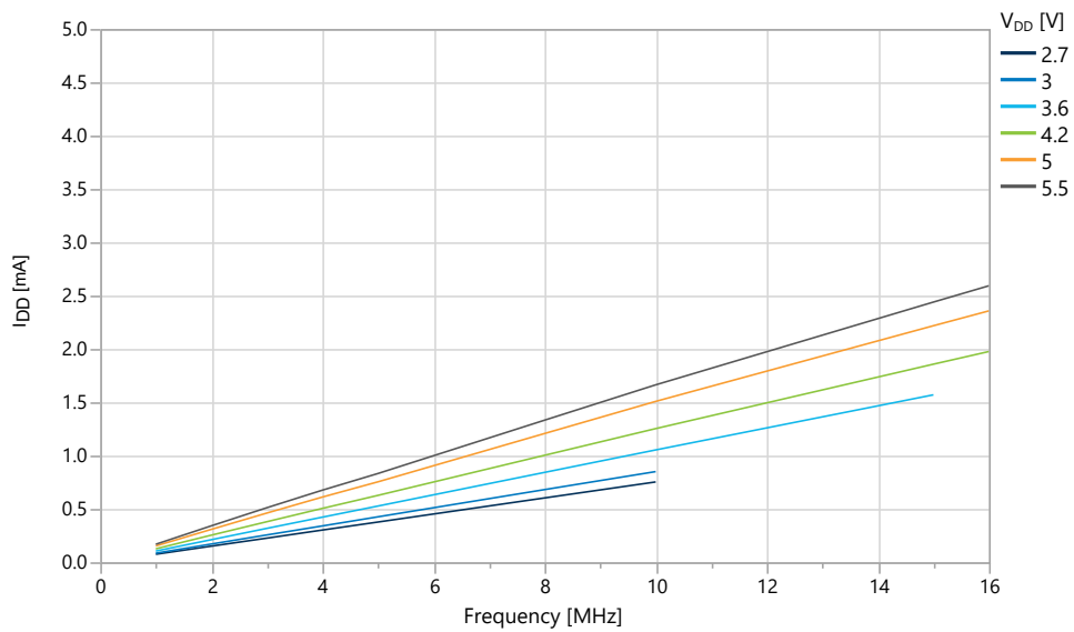
Figure 38-6. Idle Supply Current vs. Frequency (1-16 MHz) at T = 25^{\circ}C
