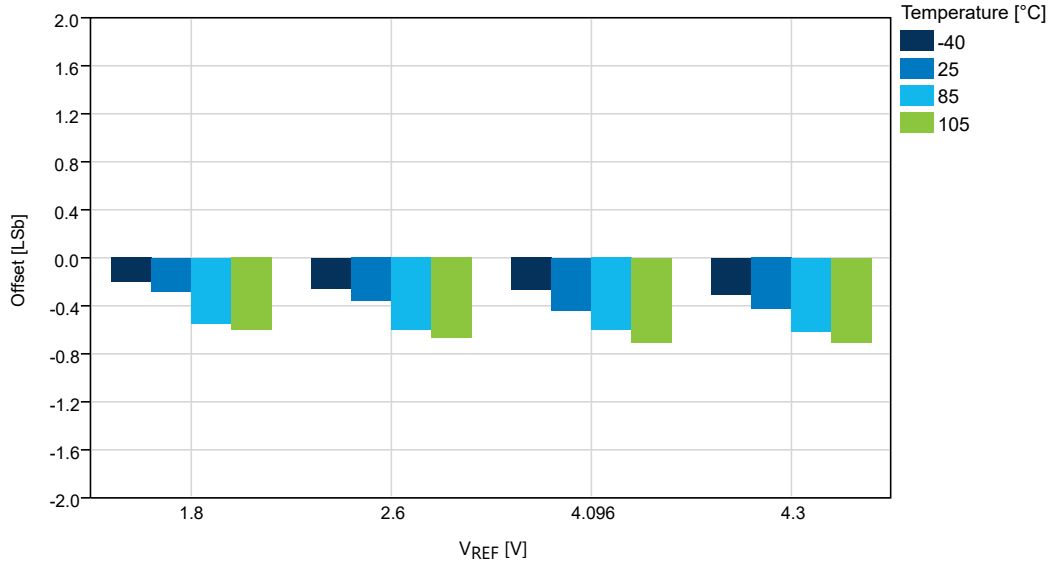
Figure 38-55. Offset vs. V_{REF} ( V_{DD} = 5.0V , f_{ADC} = 115 ksp/s, REFSEL = External Reference)
