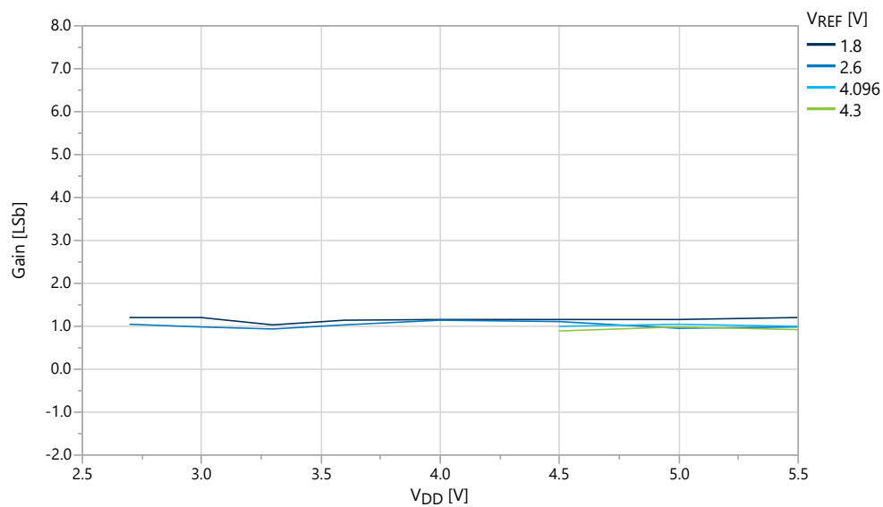
Figure 38-50. Gain vs. V_{DD} ( f_{ADC} = 115 ksp/s, T = 25^{\circ}C , REFSEL = External Reference)
