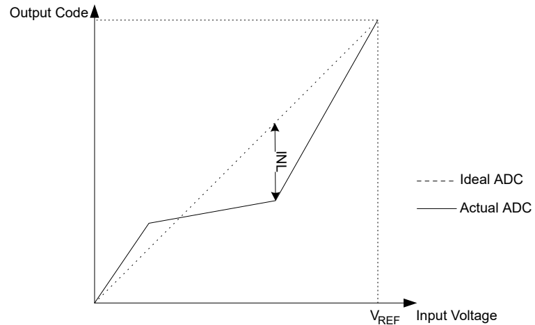
Figure 36-3. Integral Nonlinearity
