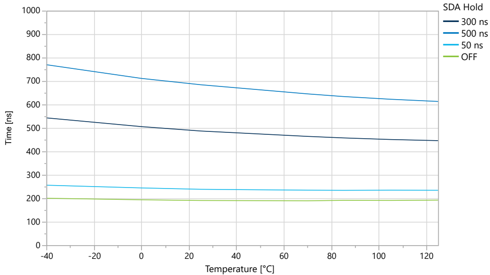
Figure 38-70. TWI SDA Hold Time vs. Temperature (Slave Mode) V_{DD} = 3V , CLK_{CPU} = 10\text{ MHz}
