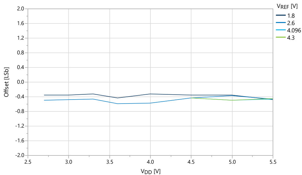
Figure 38-54. Offset vs. V_{DD} ( f_{ADC} = 115 kps, T = 25^{\circ}C , REFSEL = \text{External Reference} )
