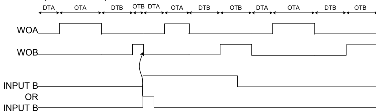
Figure 23-22. Input Mode 8 on Input B
