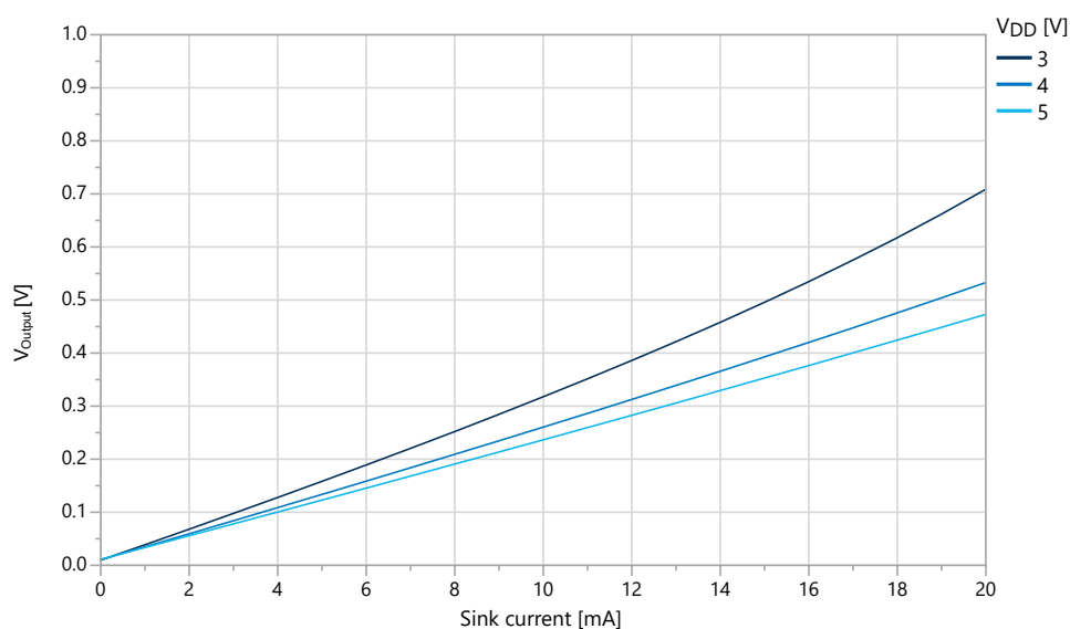
Figure 38-21. I/O Pin Output Voltage vs. Sink Current ( T = 25^{\circ}\text{C} )
