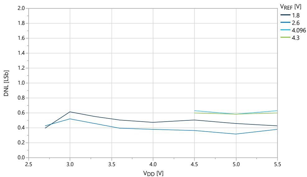
Figure 38-48. DNL vs. V_{DD} ( f_{ADC} = 115 kps, T = 25^{\circ}C , REFSEL = External Reference)
