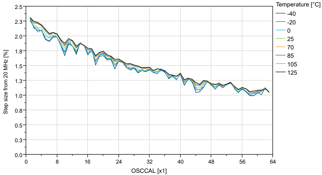
Figure 38-64. OSC20M Internal Oscillator: Calibration Stepsize vs. Calibration Value ( V_{DD} = 3V )
