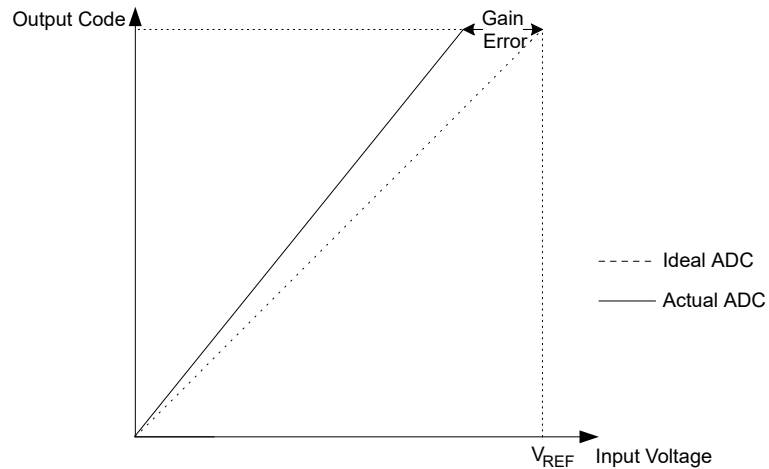
Figure 36-2. Gain Error
