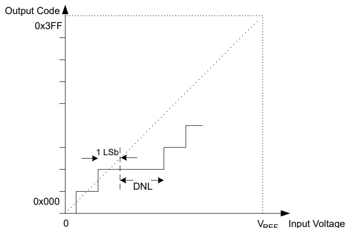
Figure 31-5. Differential Nonlinearity
