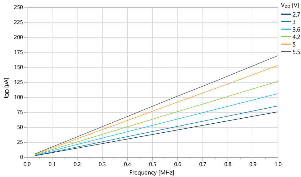
Figure 38-7. Idle Supply Current vs. Low Frequency (0.1-1.0 MHz) at T = 25°C
