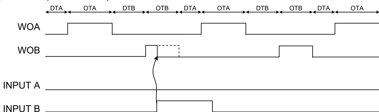
Figure 23-24. Input Mode 9 on Input B
