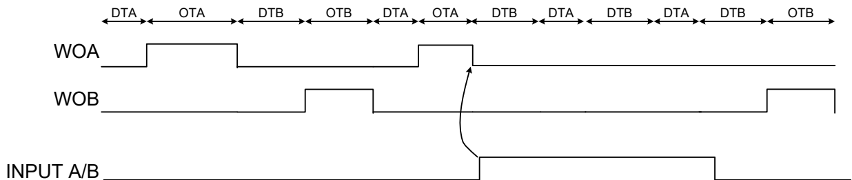
Figure 23-18. Input Mode 5
