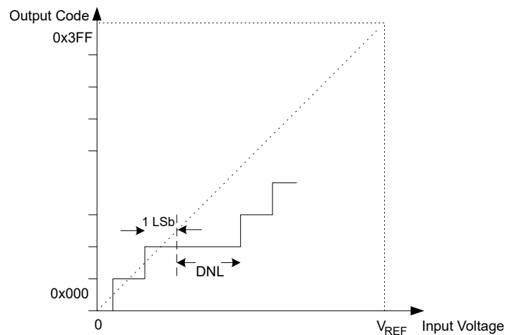
Figure 36-4. Differential Nonlinearity
