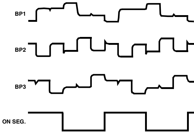
FIGURE 9. TYPICAL BACKPLANE AND ANNUNCIATOR DRIVE WAVEFORM
