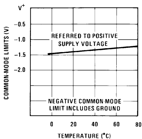
Common-Mode Limits
