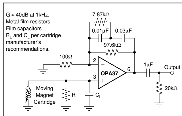
FIGURE 7. Low-Noise RIAA Preamplifier.
