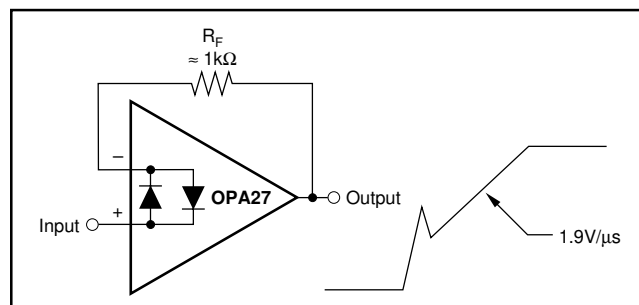
FIGURE 6. Pulsed Operation.
