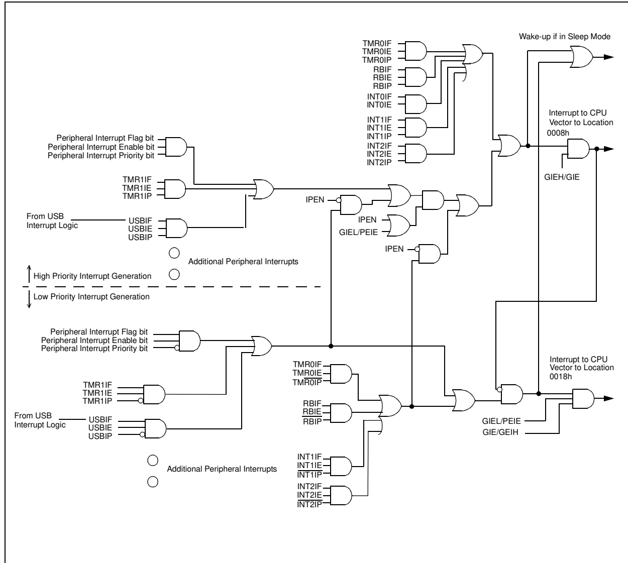
FIGURE 9-1: INTERRUPT LOGIC
