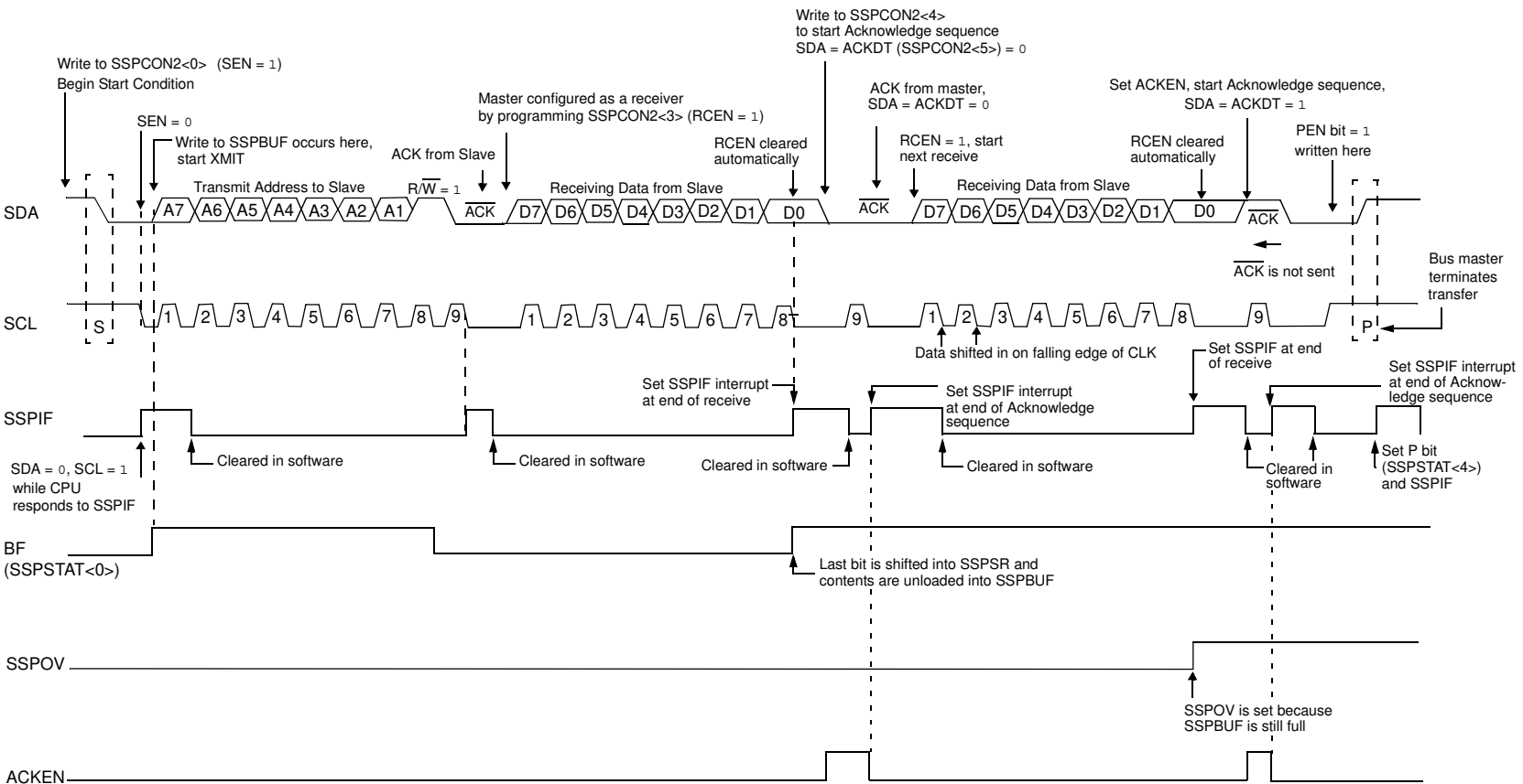
FIGURE 19-22: I 2 C™ MASTER MODE WAVEFORM (RECEPTION, 7-BIT ADDRESS)
