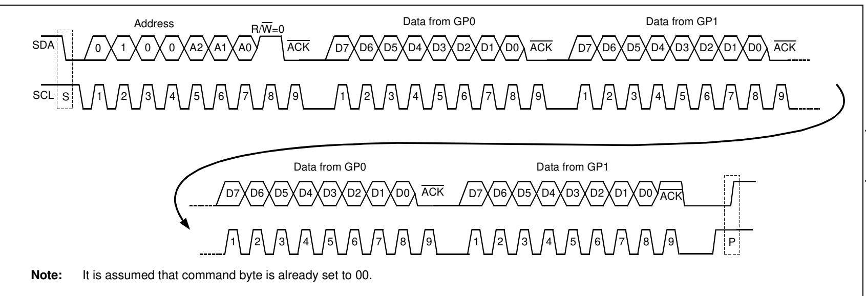
READ FROM INPUT PORTS (CASE 2)
