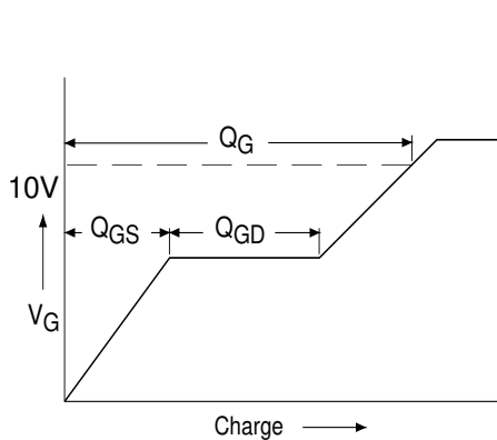
Fig 12a. Basic Gate Charge Waveform
