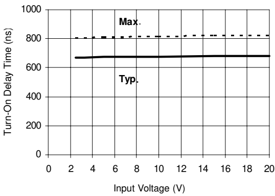
Figure 6C. Turn-On Time vs Input Voltage
