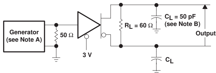
TEST CIRCUIT
