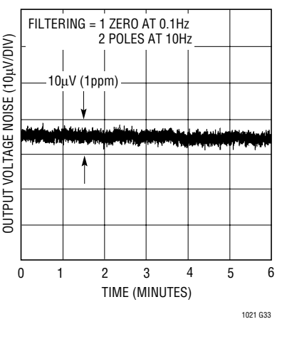
Output Noise 0.1Hz to 10Hz LT1021-10
