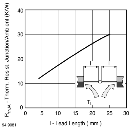
Figure 1. Typ. Thermal Resistance vs. Lead Length
