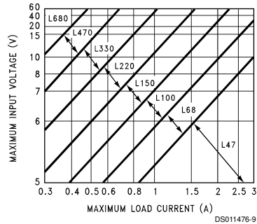
FIGURE 3. LM2576(HV)-3.3
