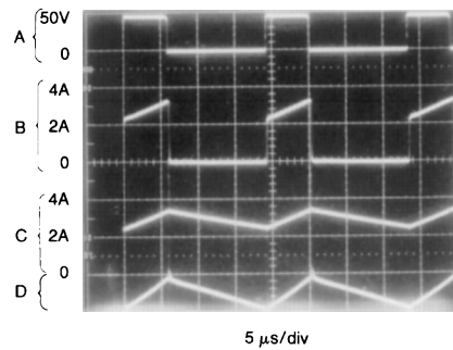
Switching Waveforms
