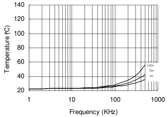
Figure 25. R21814 vs. Frequency (RFBC 20), R_{gate}=33\Omega, V_{CC}=15V
