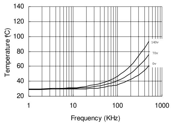
Figure 23. IR2181 vs. Frequency (RFBC 40), R_{gate}=15\Omega , V_{cc}=15V
