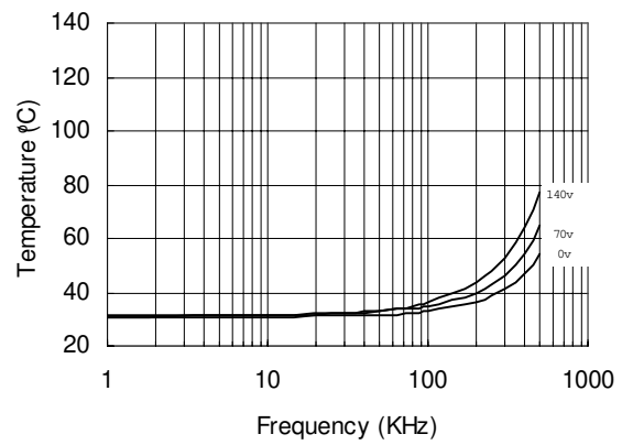
Figure 29. R2181s vs. Frequency (IRFBC 20), R_{gate}=33\Omega , V_{CC}=15V
