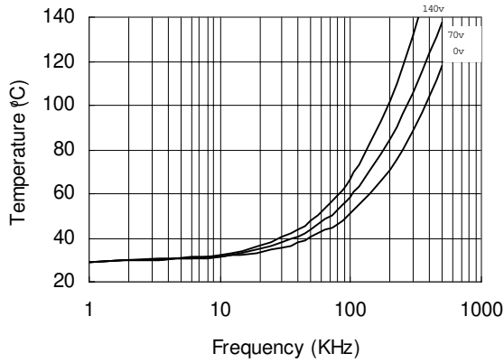
Figure 24. R2181 vs. Frequency (RFPE50), R_{gate}=10\Omega, V_{CC}=15V
