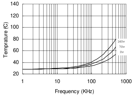
Figure 21. IR2181 vs. Frequency (RFBC 20), R_{gate}=33\Omega , V_{cc}=15V
