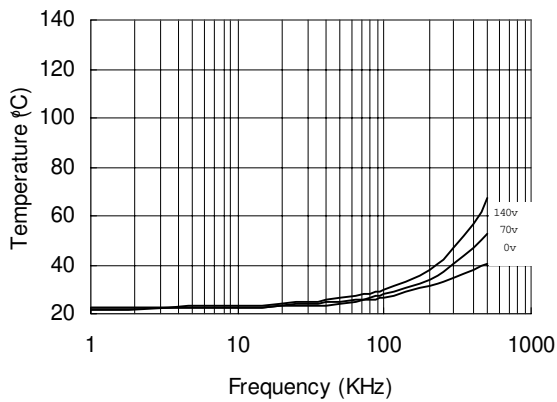
Figure 26. R21814 vs. Frequency (RFBC 30), R_{gate}=22\Omega, V_{CC}=15V
