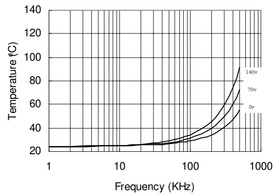
Figure 27. R21814 vs. Frequency (RFBC 40), R_{gate}=15\Omega, V_{CC}=15V
