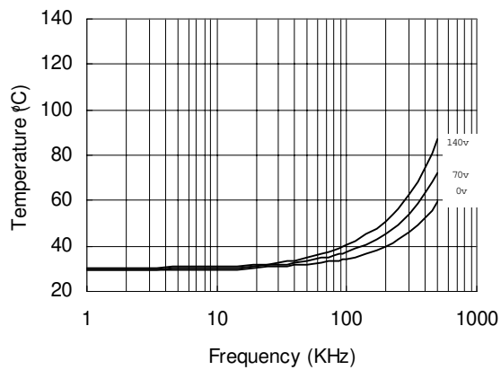
Figure 22. IR2181 vs. Frequency (RFBC 30), R_{gate}=22\Omega , V_{cc}=15V
