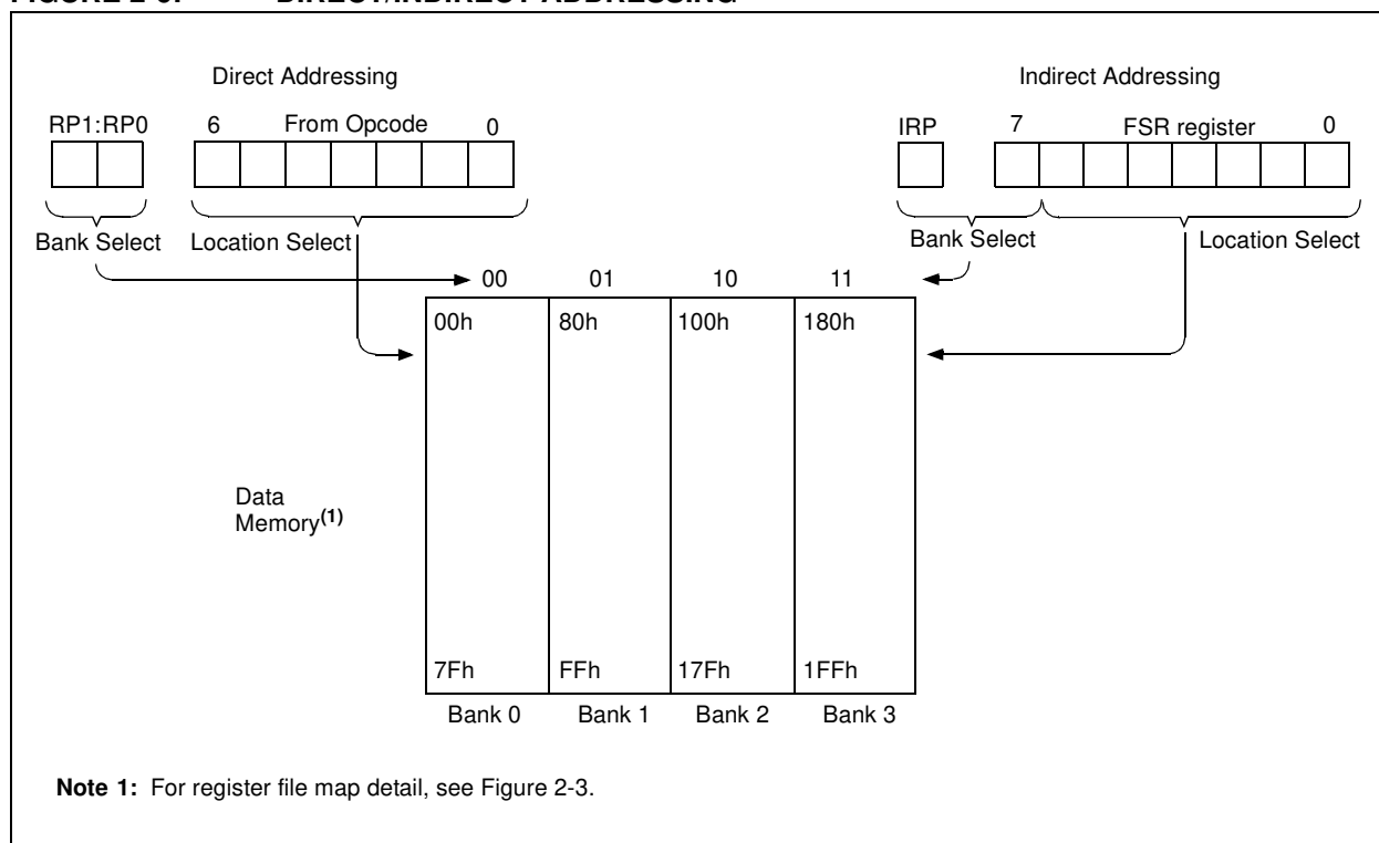
FIGURE 2-6: DIRECT/INDIRECT ADDRESSING
