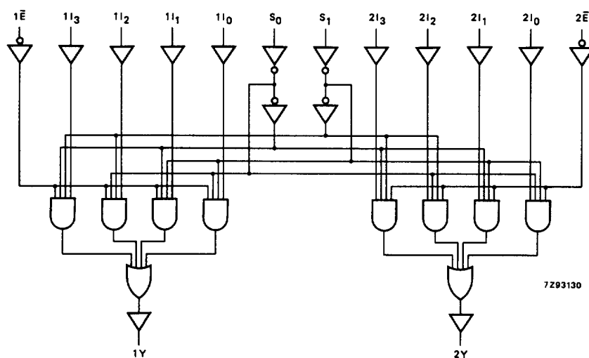
Fig.5 Logic diagram.
