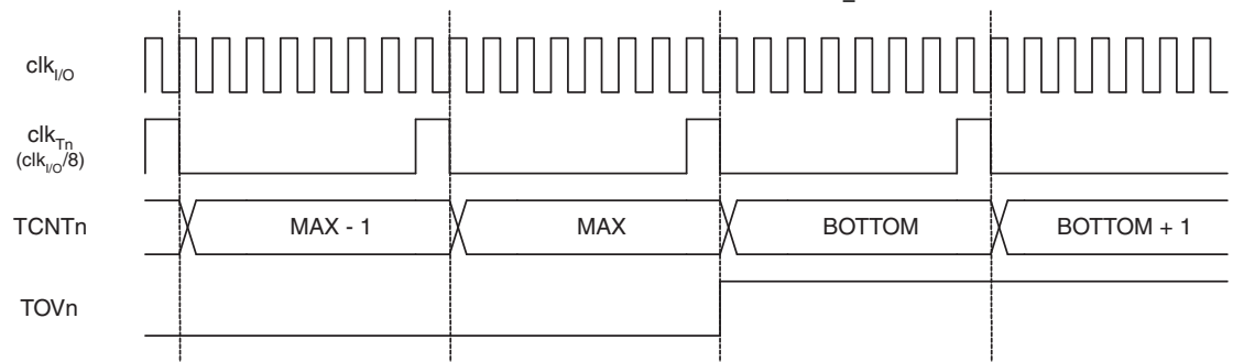
Figure 11-9. Timer/Counter Timing Diagram, with Prescaler ( f_{\text{clk\_I/O}}/8 )
