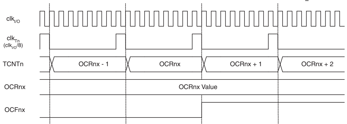
Figure 11-10. Timer/Counter Timing Diagram, Setting of OCF0x, with Prescaler ( f_{\text{clk\_I/O}}/8 )
