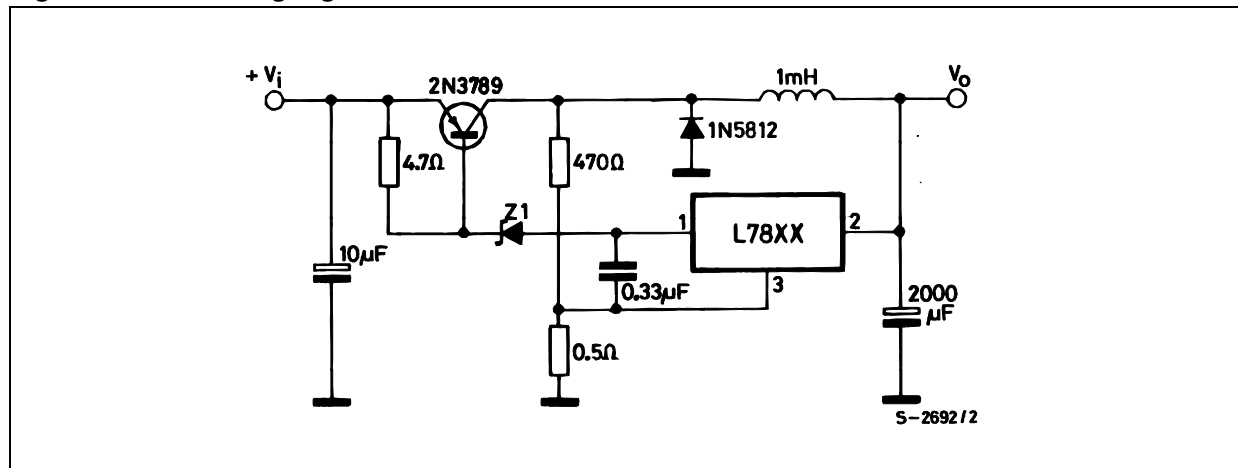
Figure 22. Switching regulator
