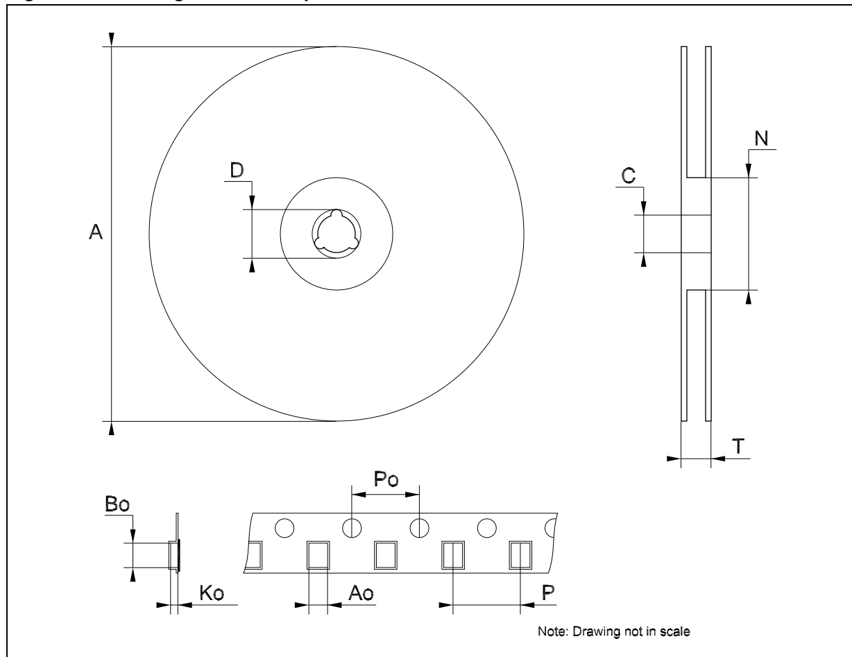
Figure 49. Drawing dimension tape and reel for DPAK
