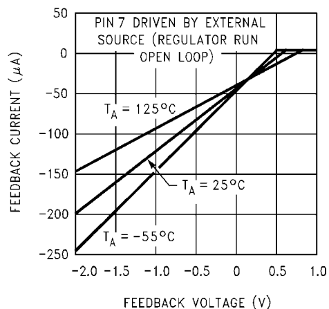
LP2951 Feedback Pin Current
