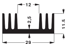
SK 09 20 TO 220
