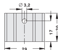
SK 145 20 TO 220
