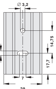
SK 145 50 TO 220
