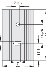
SK 09 50 TO 220
