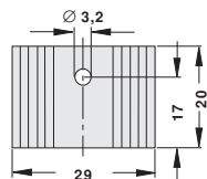
SK 09 20 TO 220
