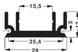
SK 145 20 TO 220
