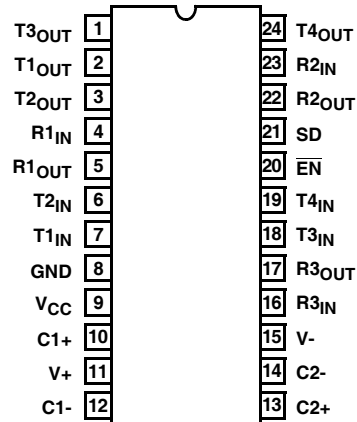
HIN236 (24 LD SOIC) TOP VIEW
