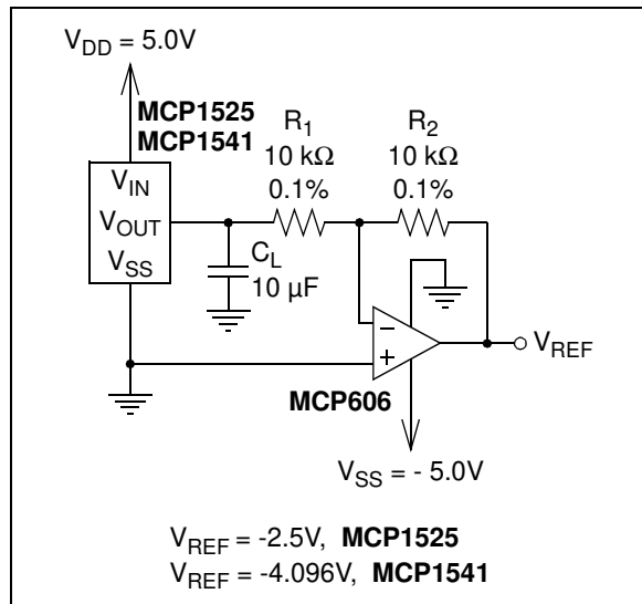
FIGURE 4-3: Negative Voltage Reference.
