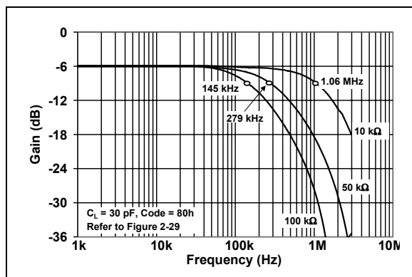
FIGURE 2-21: -3 dB Bandwidths.
