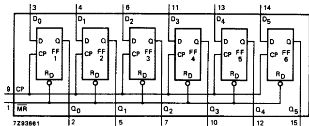
Fig.4 Functional diagram.
