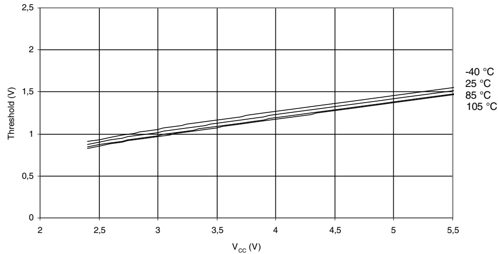
Figure 27-20. I/O Pin Input Threshold Voltage vs. V_{CC} (VIL, I/O Pin Read As '0') I/O PIN (including PE1 & PE2) INPUT THRESHOLD VOLTAGE vs. V_{CC} VIL, IO PIN READ AS '0'
