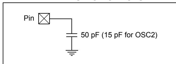
FIGURE 3-2: LOAD CONDITIONS FOR DEVICE TIMING SPECIFICATIONS
