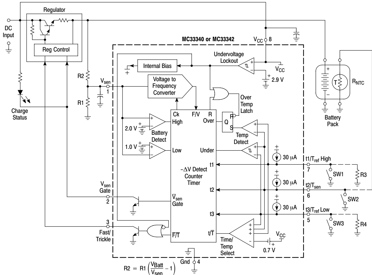
Figure 8. Typical Battery Charging Application
