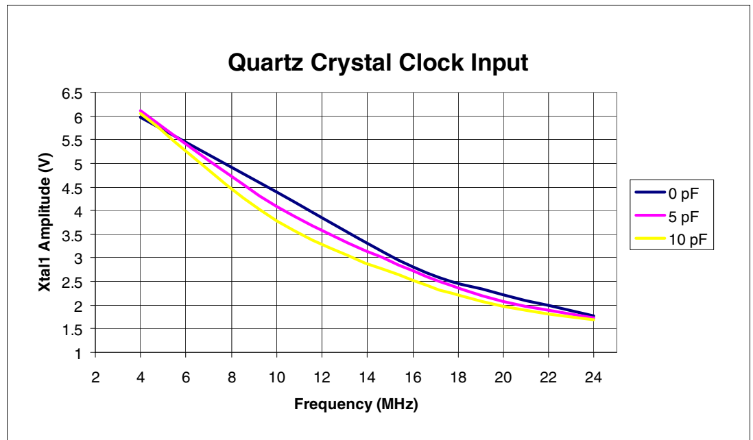
Figure 11-2. Quartz Crystal Clock Source
