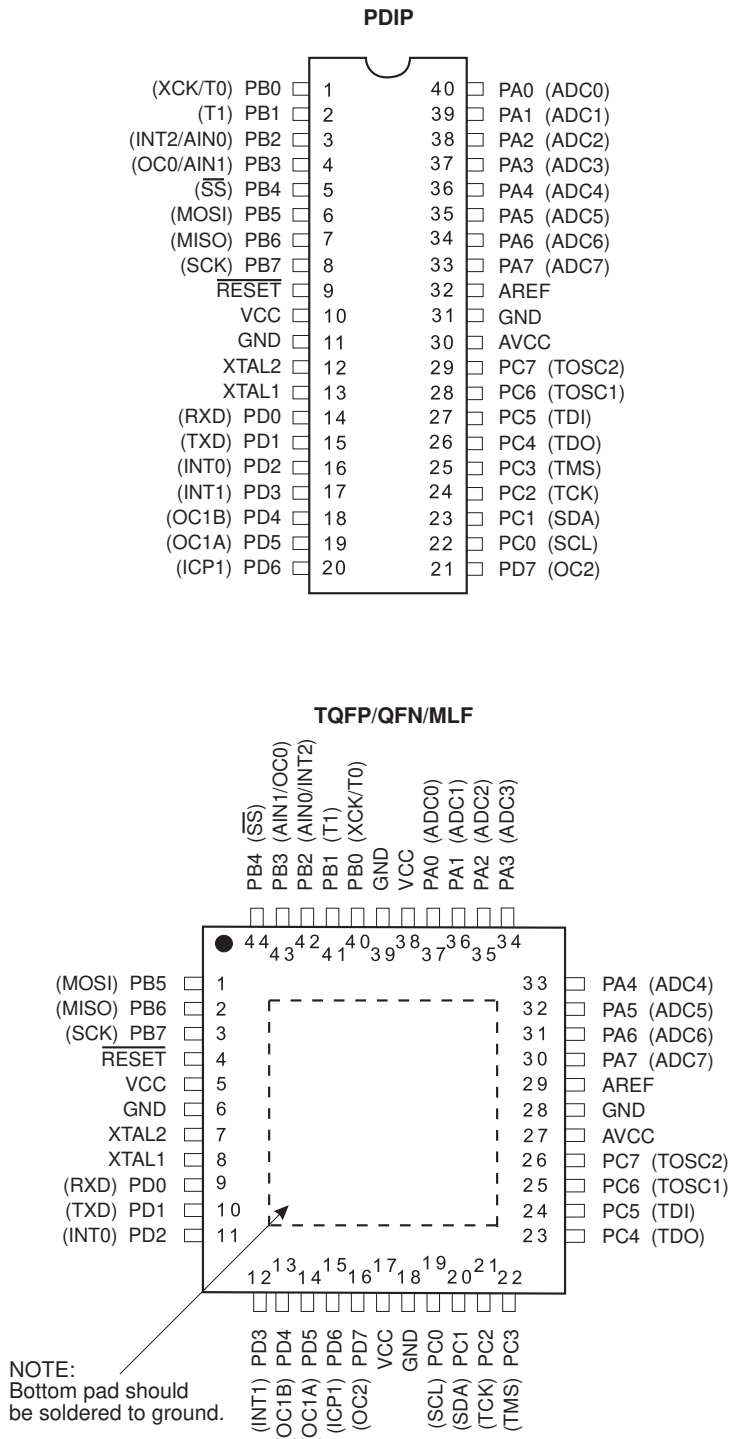
Figure 1. Pinout ATmega16
