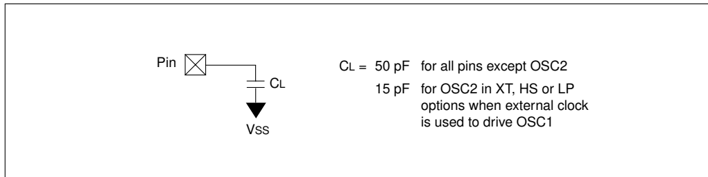
FIGURE 13-1: LOAD CONDITIONS
