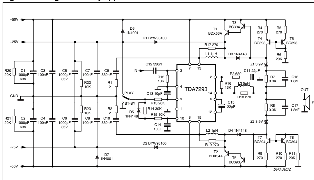
Figure 8. High-efficiency applications circuit
