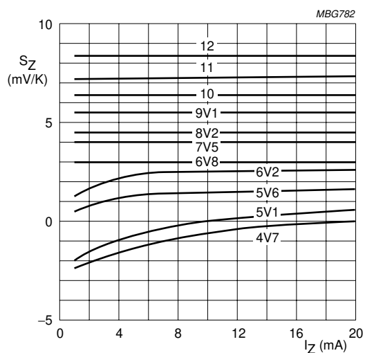
BZX84-A/B/C4V7 to A/B/C12. T_j = 25\text{ to }150\text{ }^{\circ}\text{C} .
