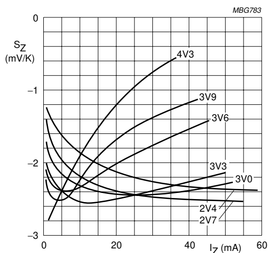
BZX84-A/B/C2V4 to A/B/C4V3. T_j = 25\text{ to }150\text{ }^{\circ}\text{C} .
