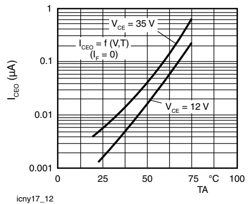
Fig. 12 - Collector Emitter Off-state Current
