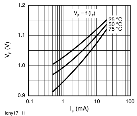
Fig. 11 - Forward Voltage
