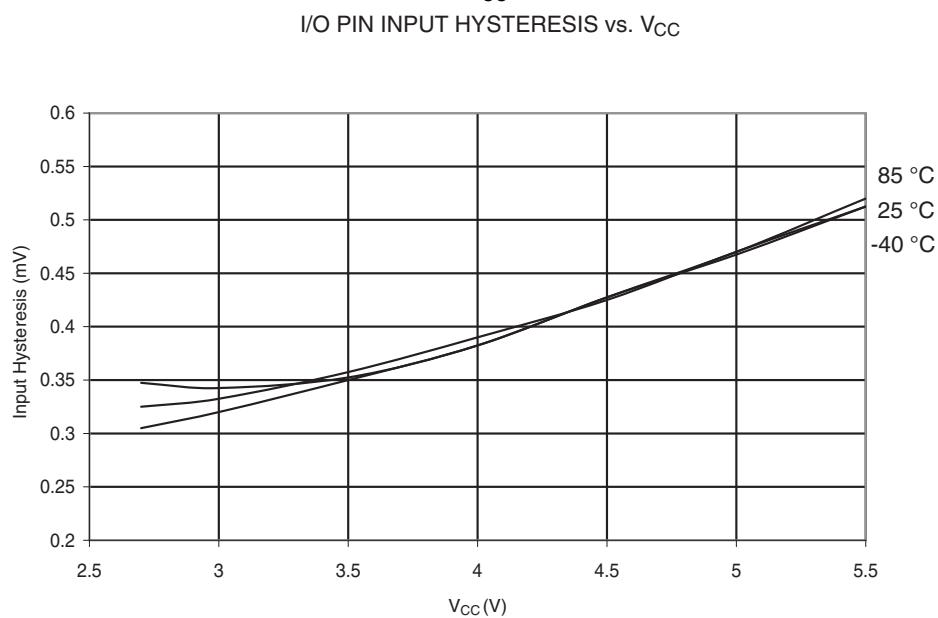
Figure 28-29. I/O Pin Input Hysteresis vs. V_{CC}
