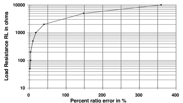
%RE vs RL at Rated primary current (AC1005)
