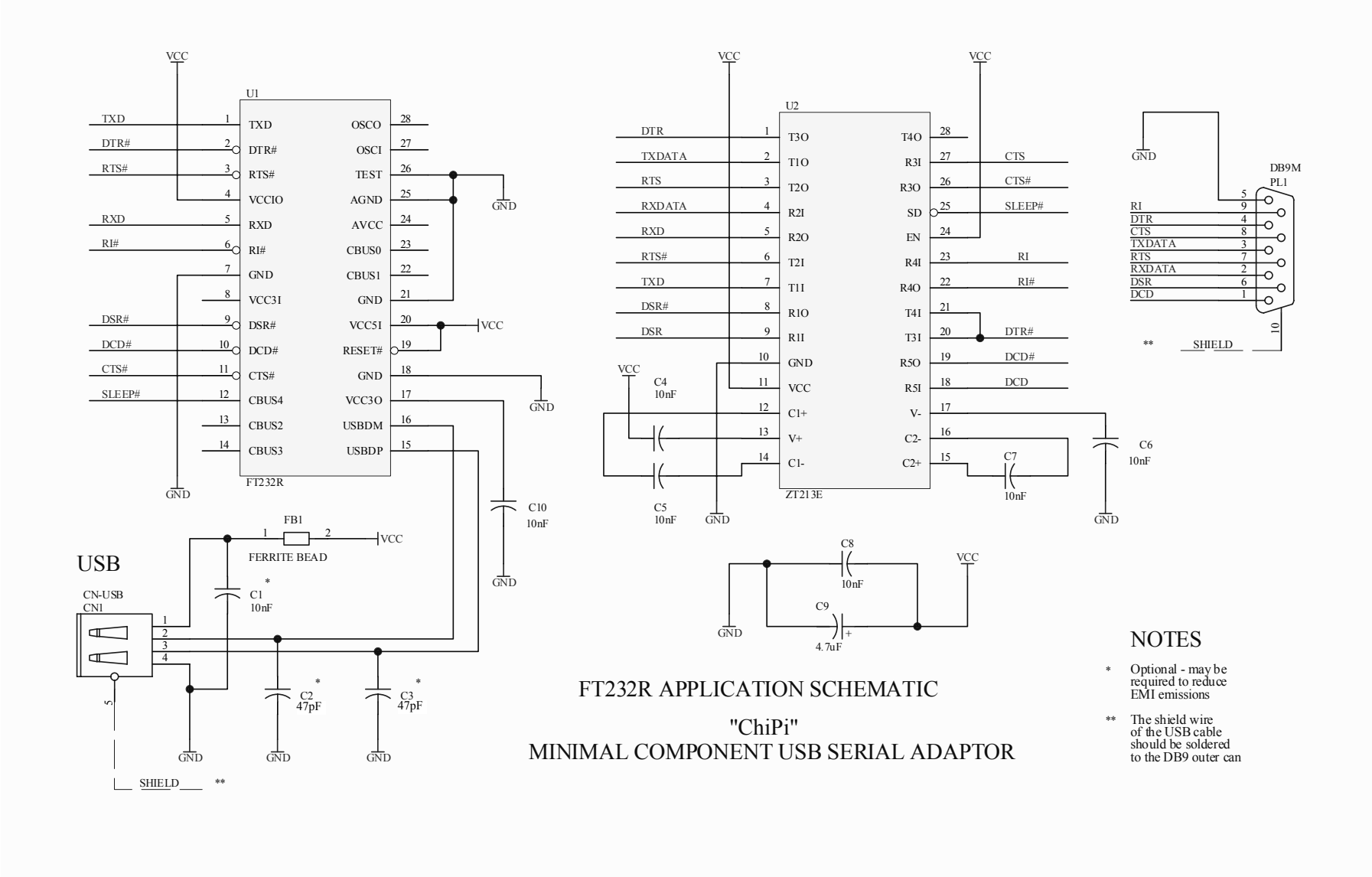
Figure 4 - UC232R "ChiPi" USB to RS232 Converter Cable Circuit Schematic
