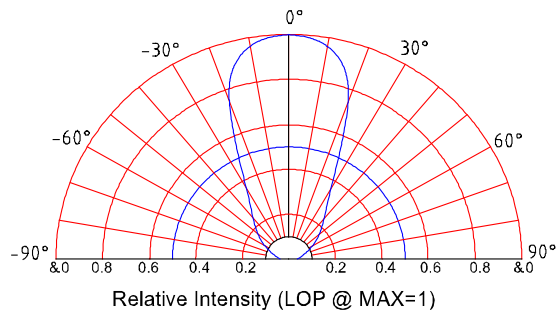
Beam Pattern
