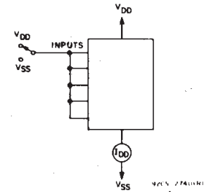
Fig. 12 - Quiescent-device-current test circuit.
