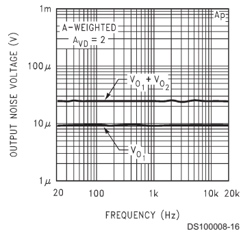
Noise Floor
