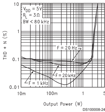
LM4871LD THD+N vs Output Power
