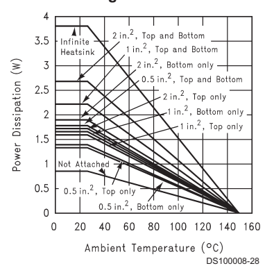
LM4871LD (Note 11) Power Derating Curve
