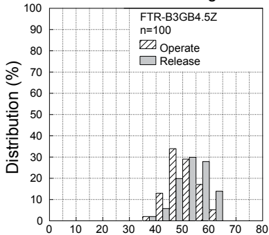
Distribution of Operate and Release Voltage
