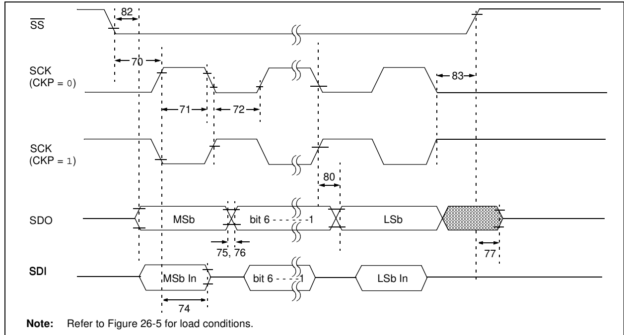
FIGURE 26-16: EXAMPLE SPI™ SLAVE MODE TIMING (CKE = 1)
