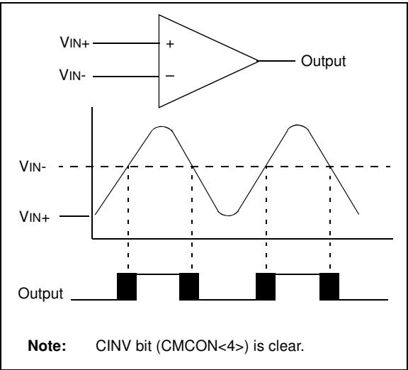
FIGURE 6-1: SINGLE COMPARATOR
