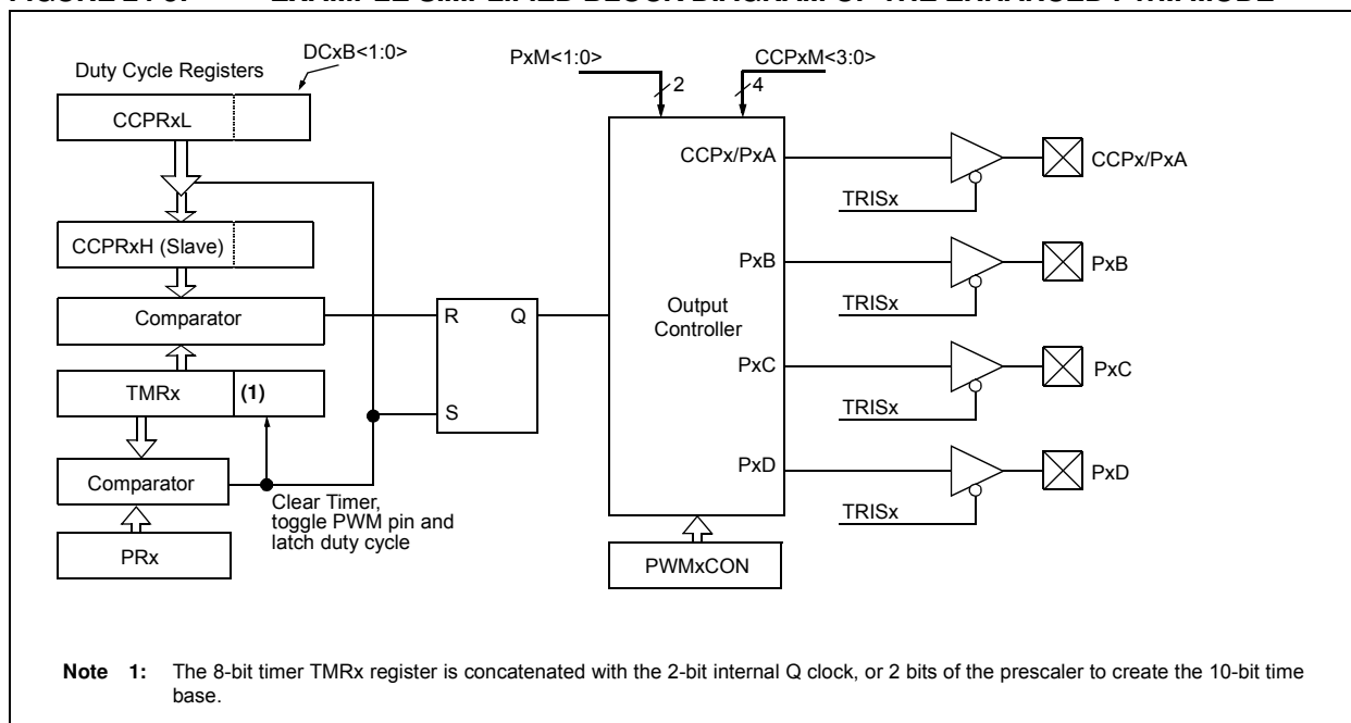
FIGURE 24-5: EXAMPLE SIMPLIFIED BLOCK DIAGRAM OF THE ENHANCED PWM MODE
