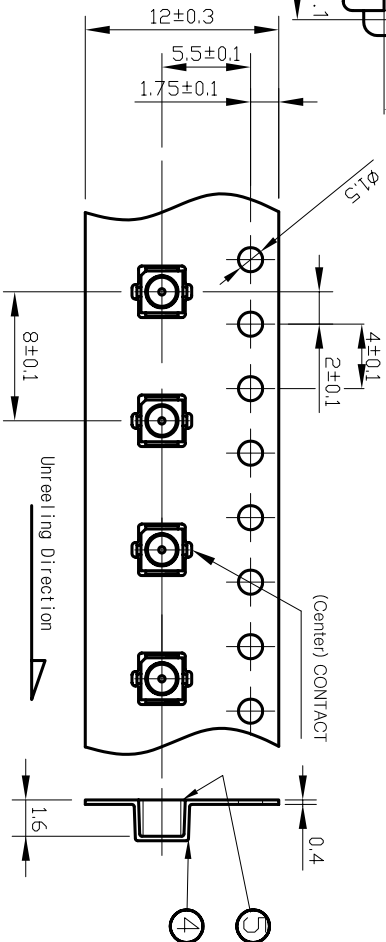
■ Embossed Tape Carrier Dimension Diagram
