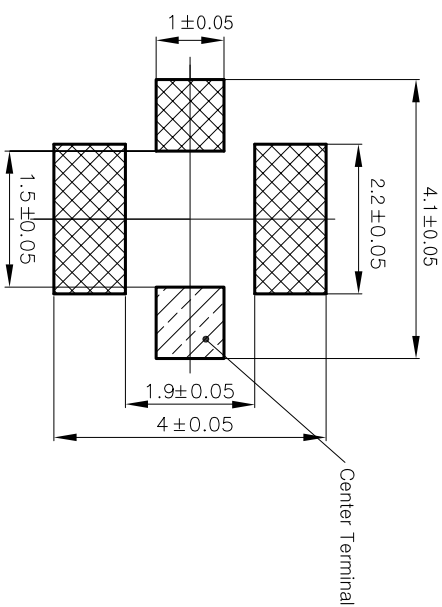
■ Recommended PCB Pattern
