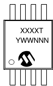
8-Lead MSOP
