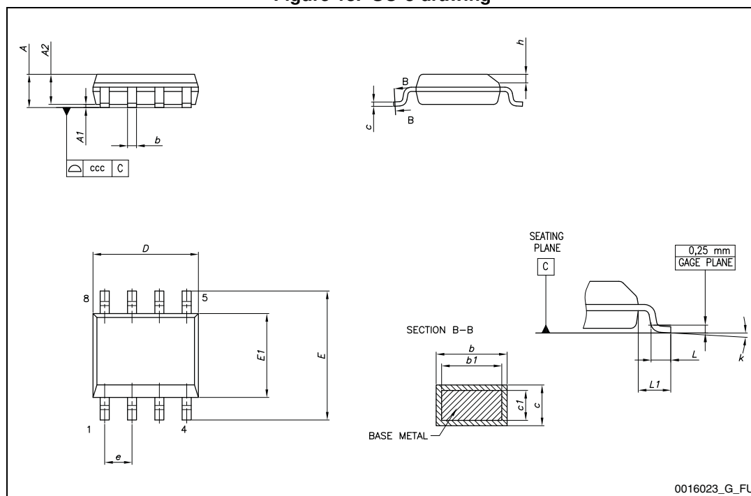
Figure 18. SO-8 drawing
