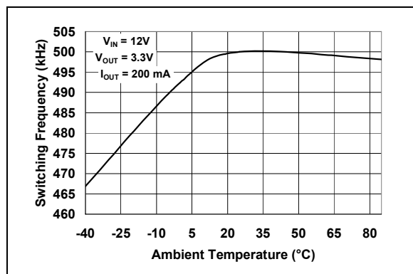
FIGURE 2-7: Switching Frequency vs. Temperature; V_{OUT} = 3.3V .
