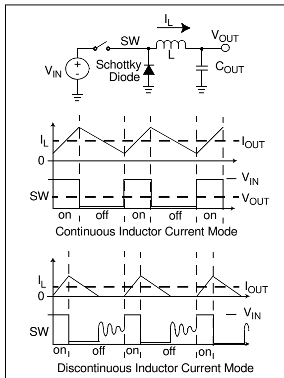
FIGURE 4-2: Step-Down Converter.
