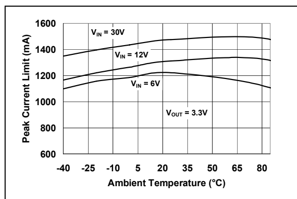
FIGURE 2-9: Peak Current Limit vs. Temperature; V_{OUT} = 3.3V .
