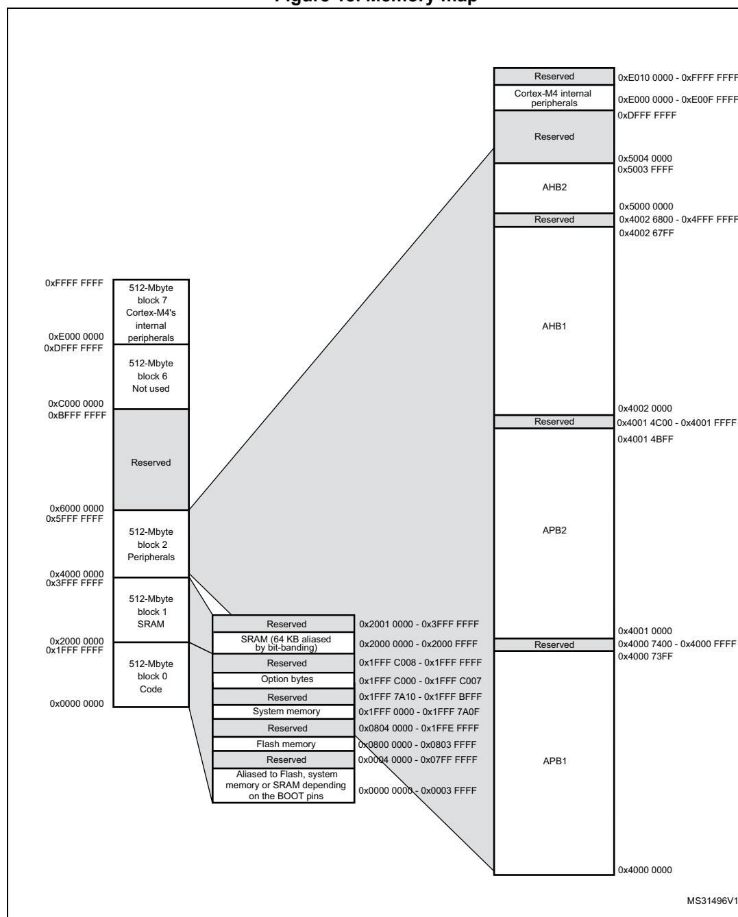
Figure 15. Memory map
