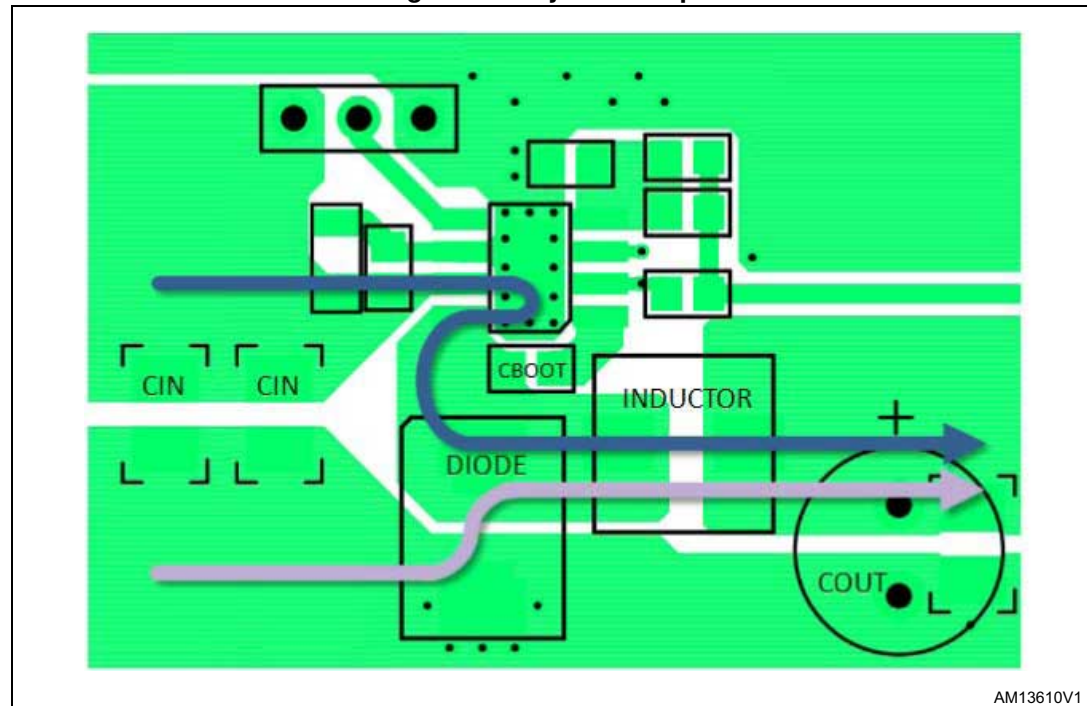
Figure 14. Layout example
