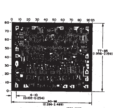
Dimensions and pad layout for CD4056BH.
