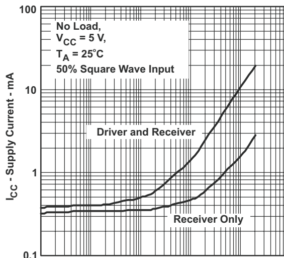
SN65HVD3088E RMS SUPPLY CURRENT vs SIGNAL RATE
